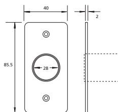
Narrow style plate dimensions
