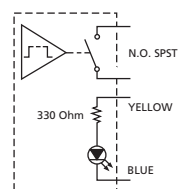
SML Switch - LED
