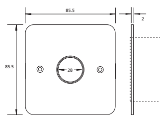
Standard MK1 gang plate dimensions
